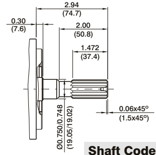
Shaft Code 11 Splined shaft Class 1-J498b 16/32 d.p 11 teeth 30° press. angle flat root side fit
